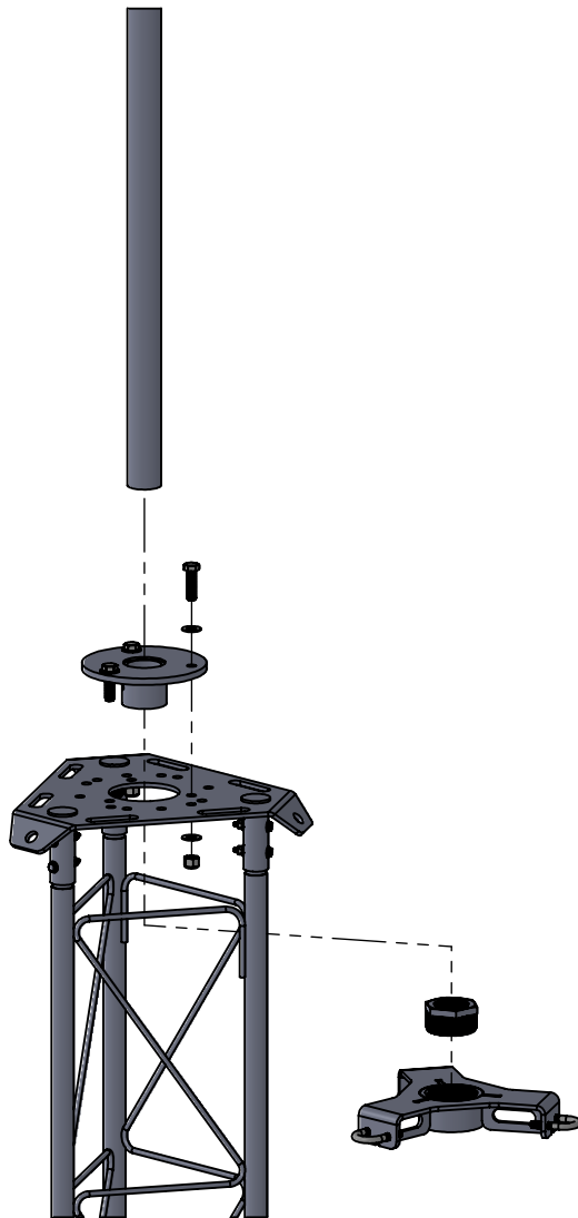
SLIP ON 1.5SCH40 PIPE
