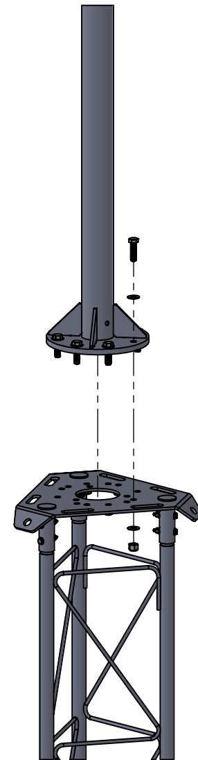
BOLT ON 2.5SCH40 PIPE
