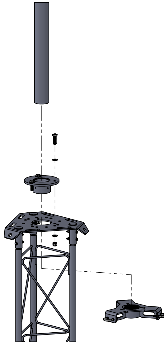
SLIP ON 2.5SCH40 PIPE
